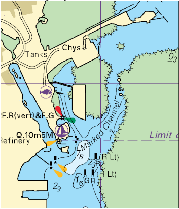
Block for Chart No 3790
